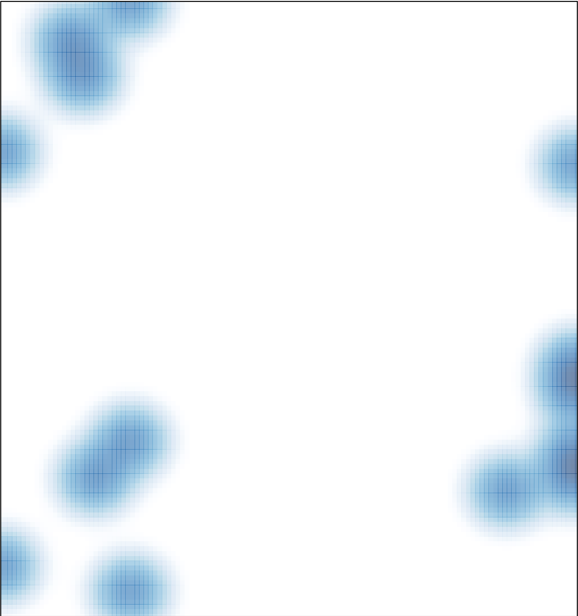
# features = 14 , max = 1
